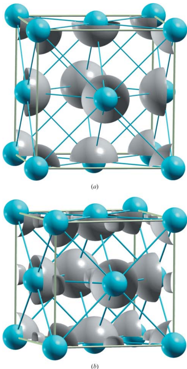
Figure 2 ELF for the fcc structure of Ca. (a) Unit cell at ambient conditions ( a = 5.521 Å) showing the charge concentration at the atomic sites. (b) Computed ELF for an fcc -Ca unit cell having the same dimension as the rocksalt CaO phase ( a = 4.829 Å). Note the formation of a charge concentration at the oxygen positions. The three-dimensional ELF plots have been generated with the help of the XcrySDen molecular structure visualization program (Kokalj, 2003), using an isovalue of 0.8 and applying the tricubic spline interpolation with a degree of three. Blue spheres represent Ca atoms.
